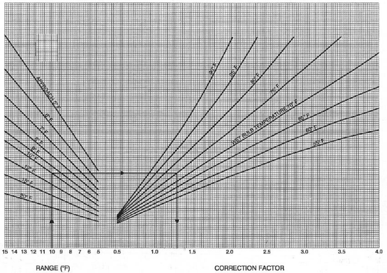
FIGURE 1. COOLING TOWER CORRECTION FACTORS
